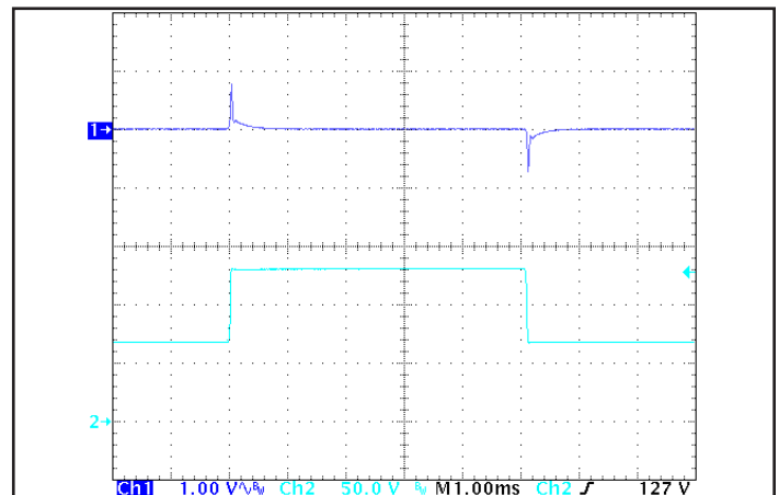
Figure 6: Output voltage response to step-change in input voltage (nominal to maximum, 250 V/ms). Load cap: 15 μF tantalum and 1 uF ceramic capacitors. Ch 1: Vout, Ch 2: Vin.
