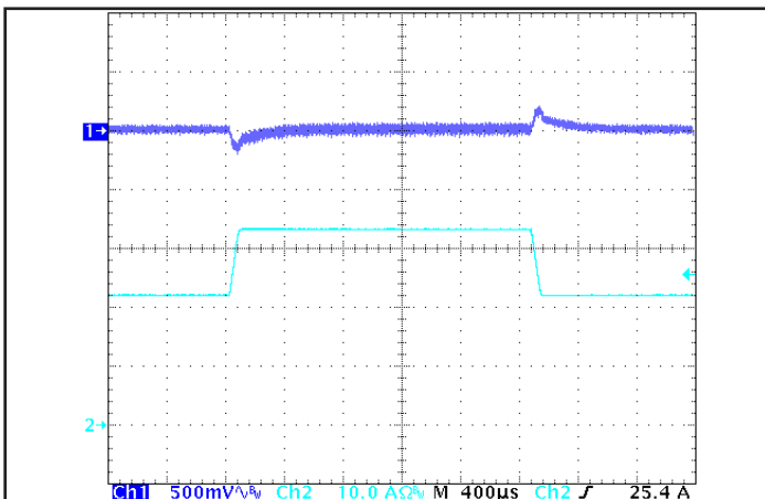
Figure 5: Output voltage response to step-change in load current (50% -75% -50% of I out (max); dI/dt = 0.2 A/μs). Load cap: 15μF tantalum and 1μF ceramic capacitors. Ch 1: V out , Ch 2: I out .
