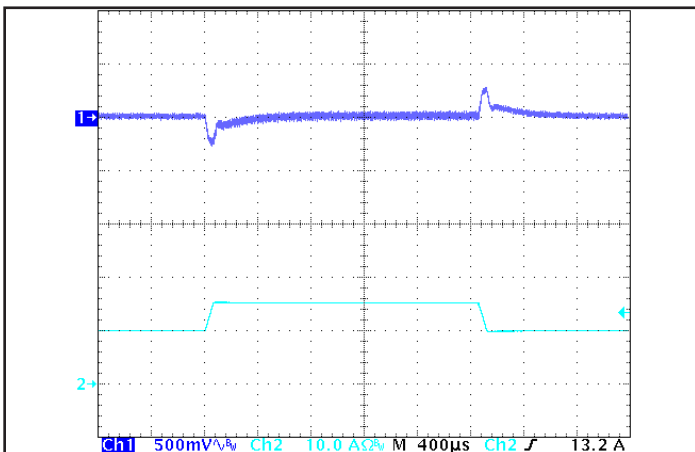
Figure 5: Output voltage response to step-change in load current (50% -75% -50% of Iout(max); dI/dt = 0.2 A/μs). Load cap: 15 μF tantalum and 1 uF ceramic capacitors. Ch 1: Vout, Ch 2: Iout.
