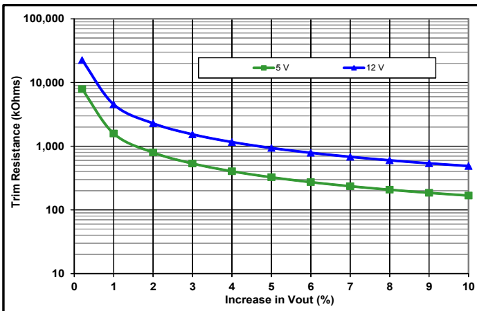
Common Figure 3: Trim graph for trim-up 5 to 12 V outputs.
