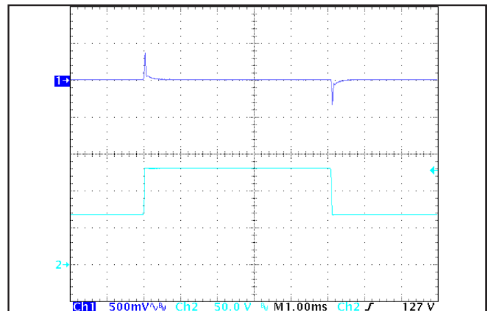
Figure 6: Output voltage response to step-change in input voltage (nominal to maximum, 250 V/ms). Load cap: 15 μF tantalum and 1 μF ceramic capacitors. Ch 1: V out , Ch 2: V in .
